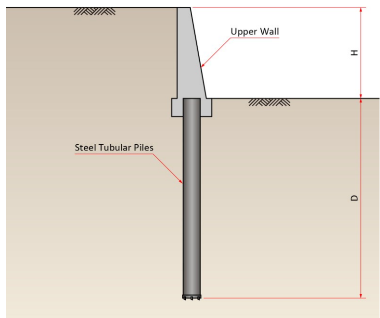
Figure 2. Cross Section (Retaining Wall)
