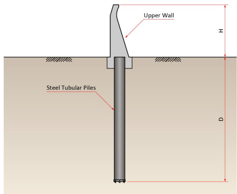
Figure 3. Cross Section (Barrier)
