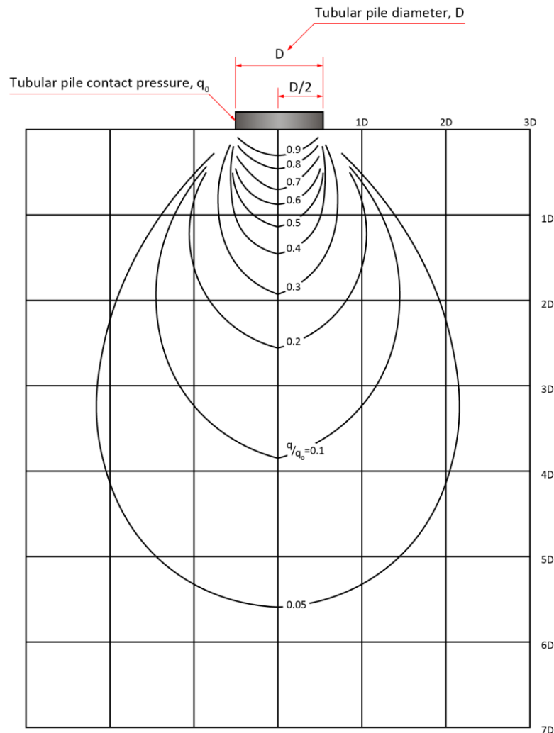
Figure 4. Pressure bulbs formed on the passive side of a tubular pile, showing the intensity of pressure q/q_0 , based on the Boussinesq equation (after Bowles [1996])
