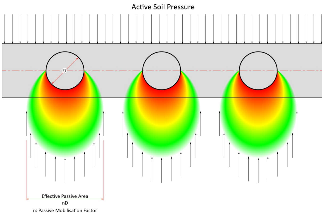
Figure 5. Schematic effective area for passive soil pressure
