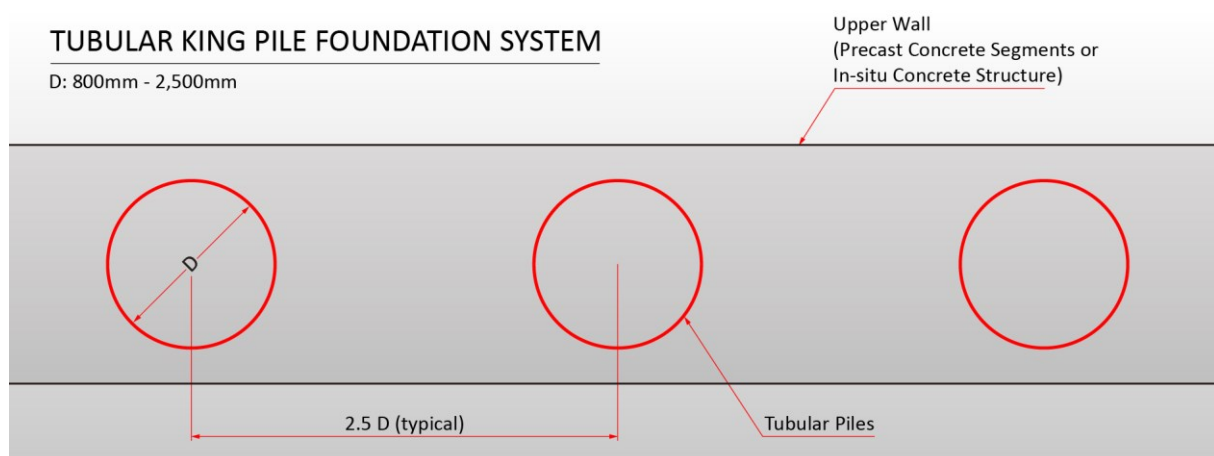
Figure 1. Foundation Configuration
