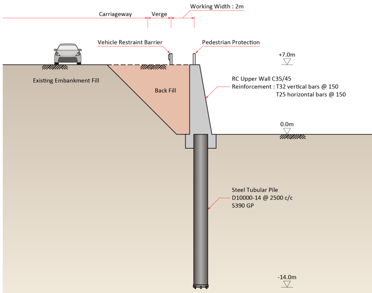
Figure 6. Section showing design of the Tubular King Pile Foundation
