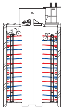
After renewal Capacity: 180 bicycles (parking/rental cycle)
